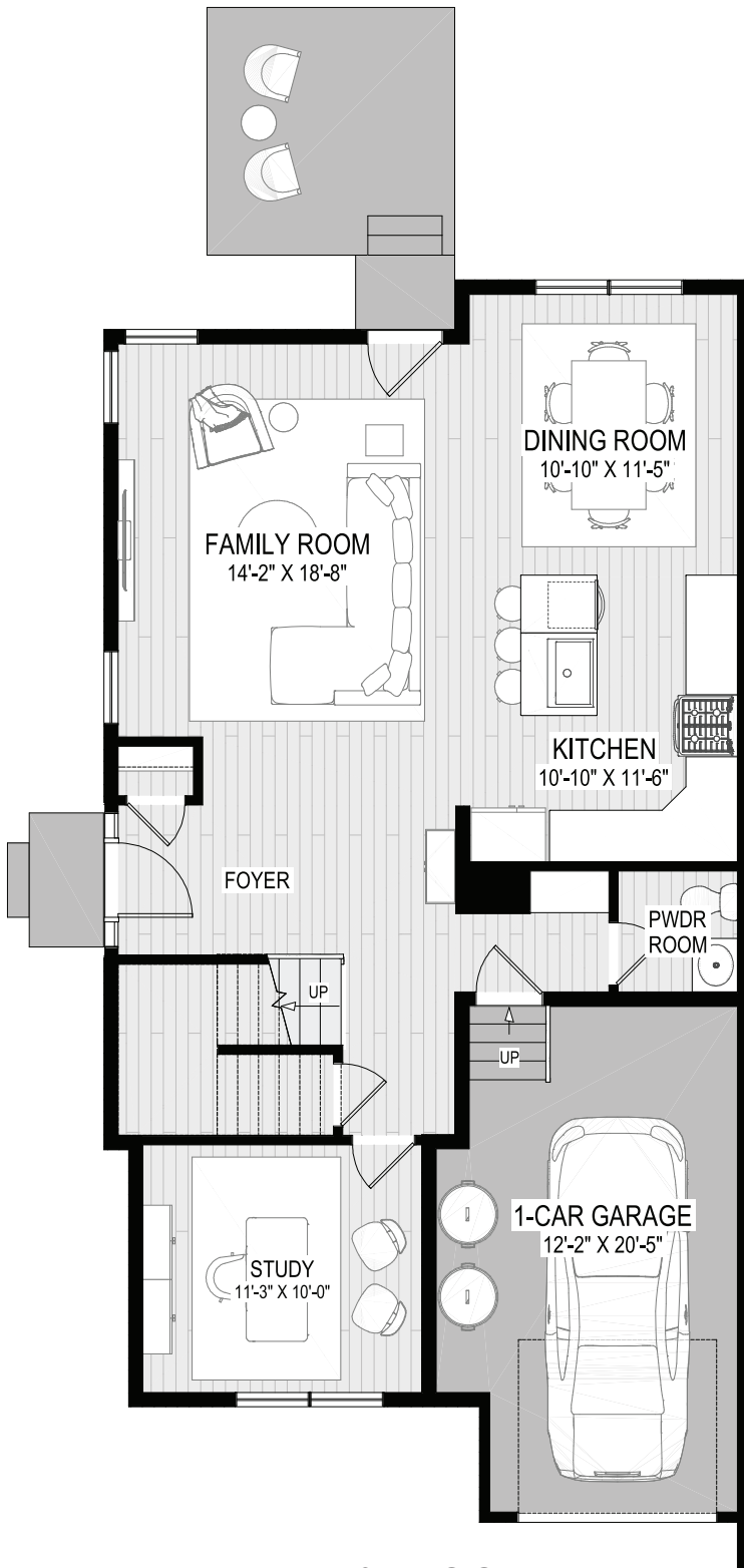
FIRST FLOOR
